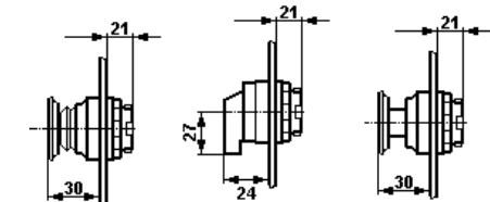
Schlagtaster "NOT-AUS" Schalter Potentiometer Schlagtaster Mushroom-head "EMERGENCY STOP" Switch Potentiometer Mushroom-head "EMERGENCY STOP"
